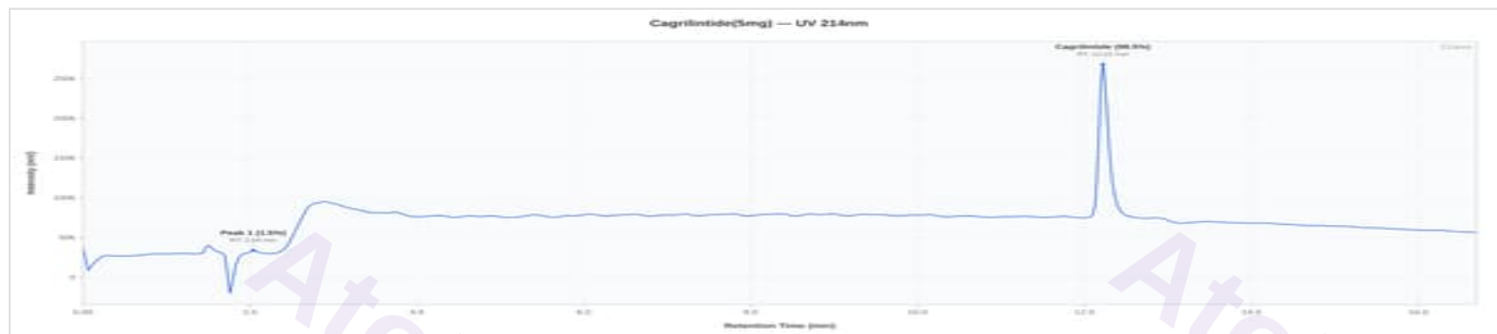
Cagrilintide 5mg - A2Z-CAGR-0000001: UV Chromatogram
